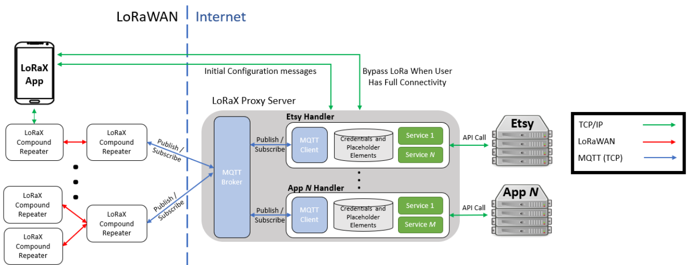
Figure 2: LoRaX network architecture.
