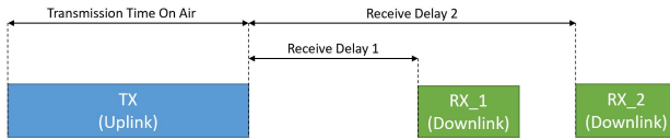
Figure 12: LoRa Class A end device timing
