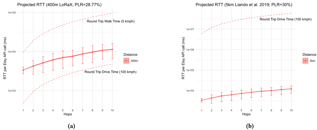
Figure 9: Projected RTT per API call relative to average drive time for the same distance to nearest Internet access point for (a) 400m hops and (b) 5km hops.
