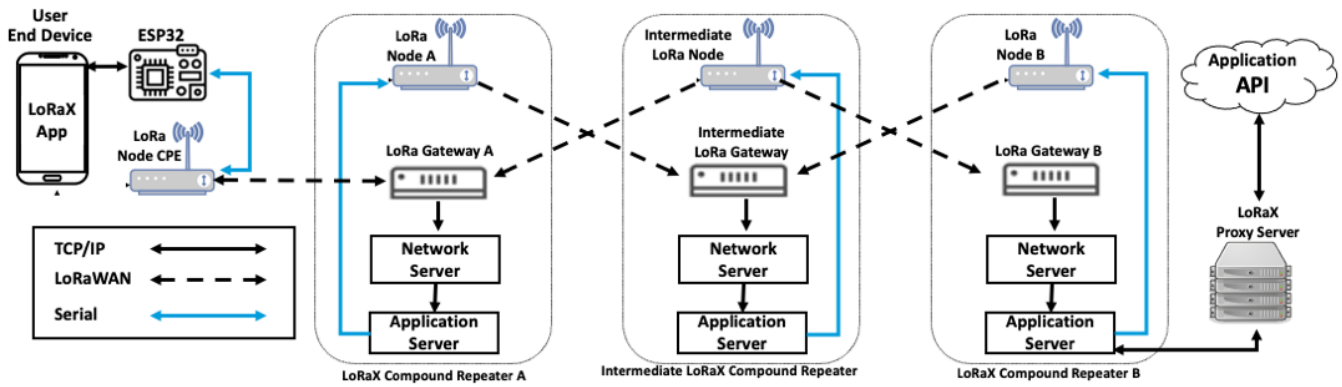
Figure 2: LoRaX network architecture.
