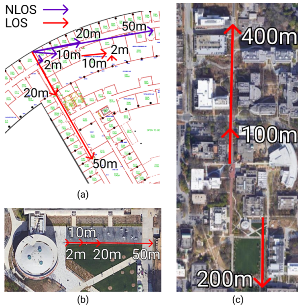
Figure 7: Measurement locations for (a) indoor tests, (b) 2-20 m outdoor tests, and (c) 100-400 m outdoor tests.
