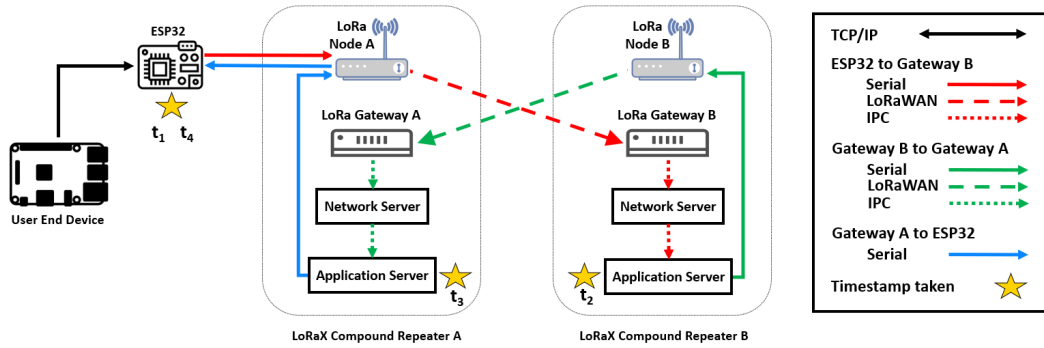
Figure 6: Measurement configuration including points (stars) where NTP-synchronized timestamps were collected.
